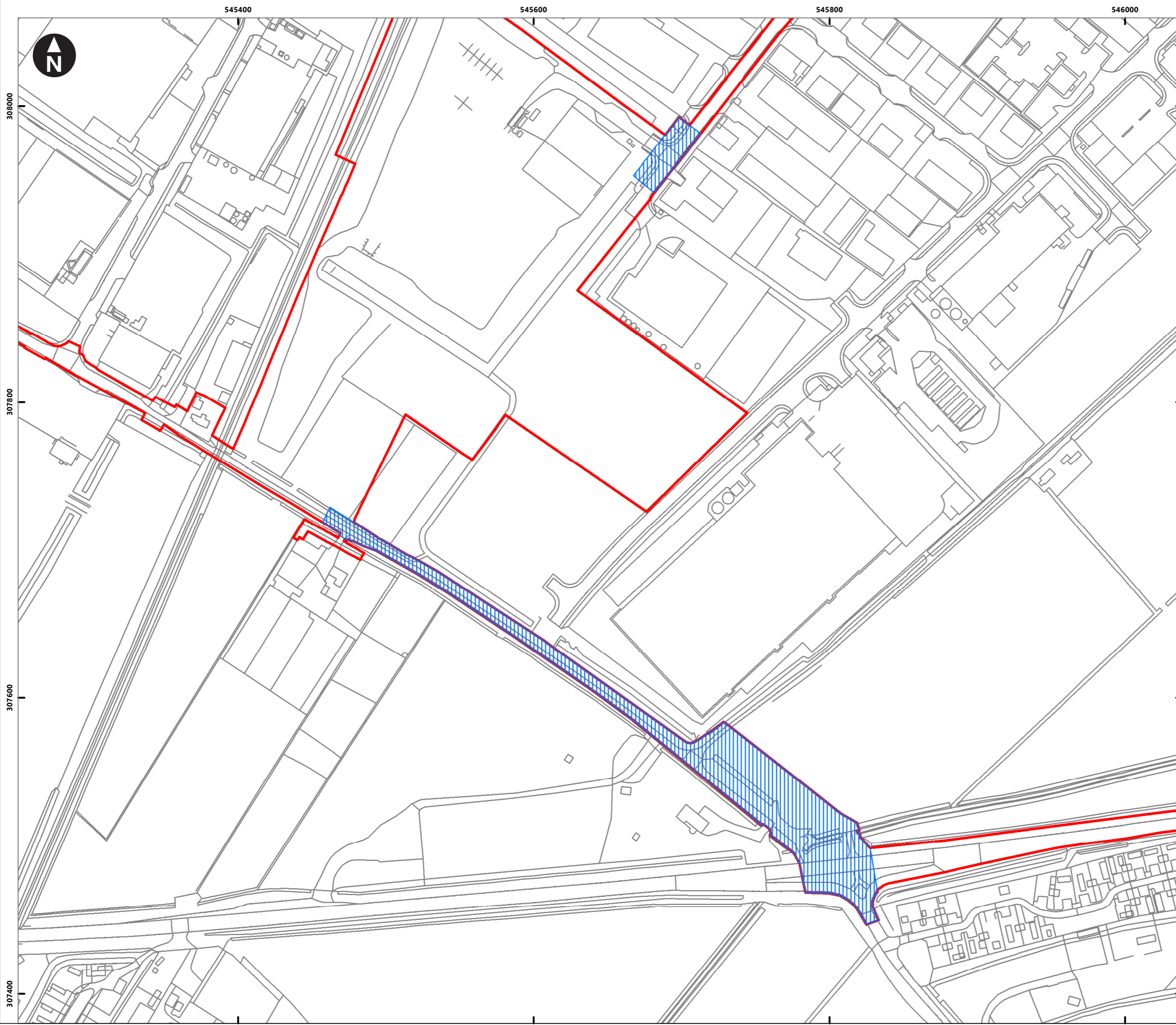
Figure 6.1 Water Connections layout
